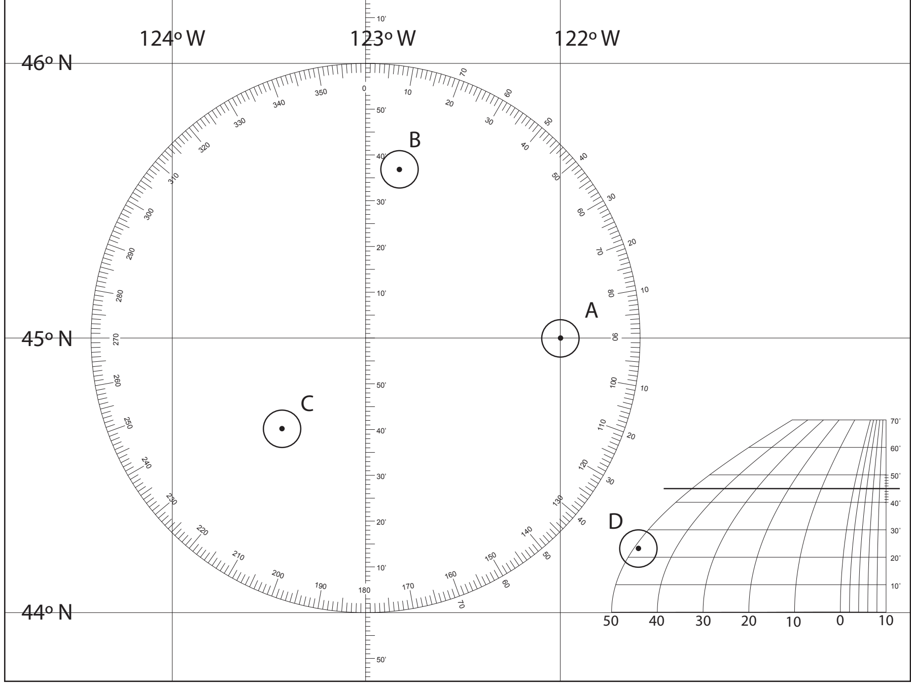
Figure 4.3-1 Plotting sheet for Exercise on universal plotting sheets, Section 4.3. This can be worked right on the page.
