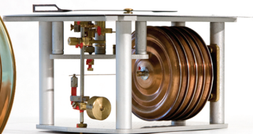
Precision movement with 5 aneroid capsules
